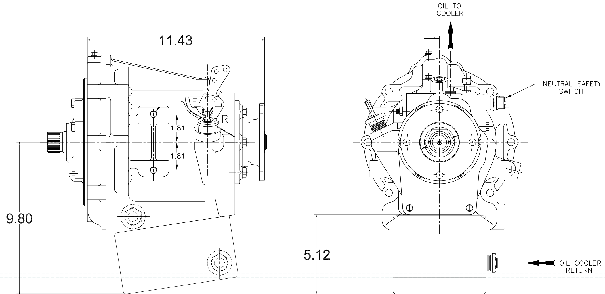
BAM Cyborg 1500 Dry Sump driveline w/ Flange
